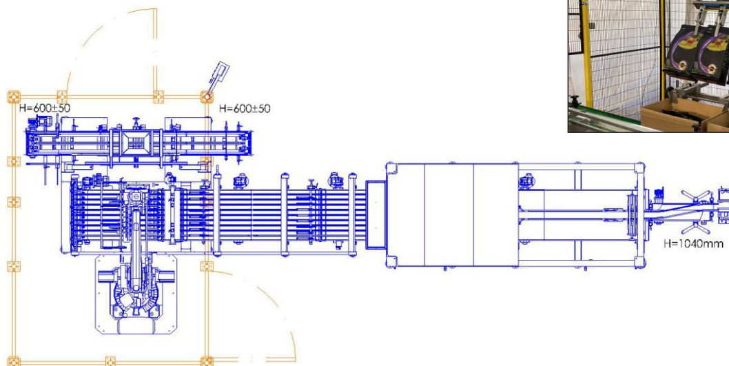
Case Packing Section
